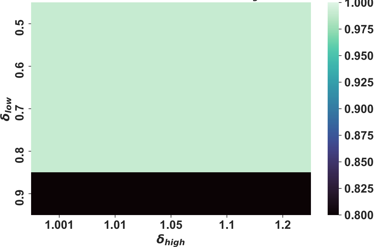
\theta_A as a function of \delta_{low} and \delta_{high}
